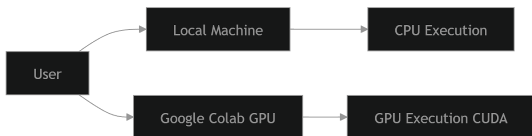
Gambar 2 Deployment Diagram
